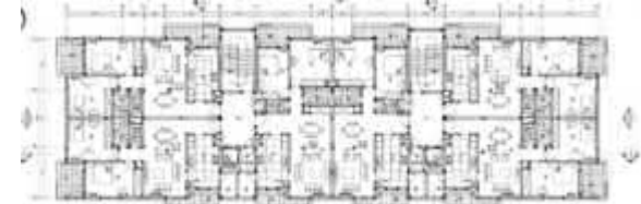
typical plan-3-3
